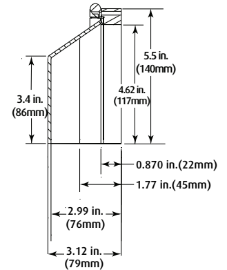
SIDE VIEW STI-6522
