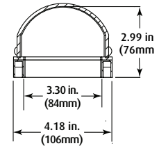
END VIEW STI-6522
