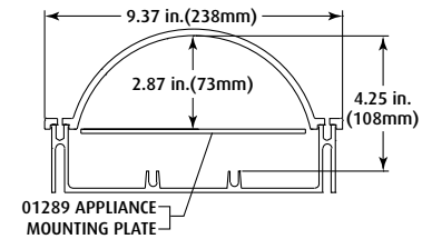
PRODUCT DIMENSIONS
