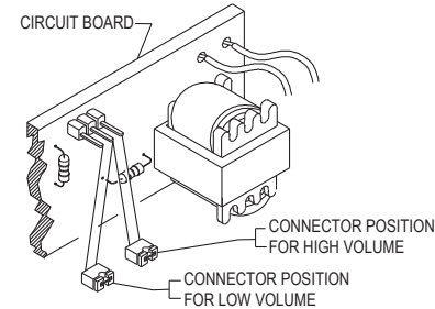
VIEW SHOWING JUMPER LOCATION FOR VOLUME SETTINGS
