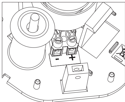
VIEW SHOWING TERMINALS FOR ELECTRICAL CONNECTION
