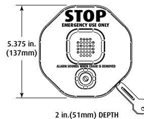
PRODUCT DIMENSIONS
