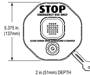
PRODUCT DIMENSIONS
