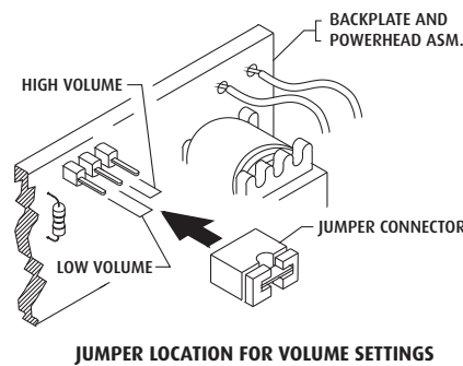
JUMPER LOCATION FOR VOLUME SETTINGS
