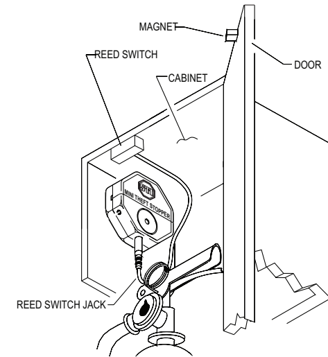
CABINET MOUNT
