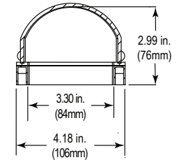
END VIEW STI-6520 STI-6521 STI-6522
