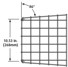
STI-9649 SIDE VIEW
