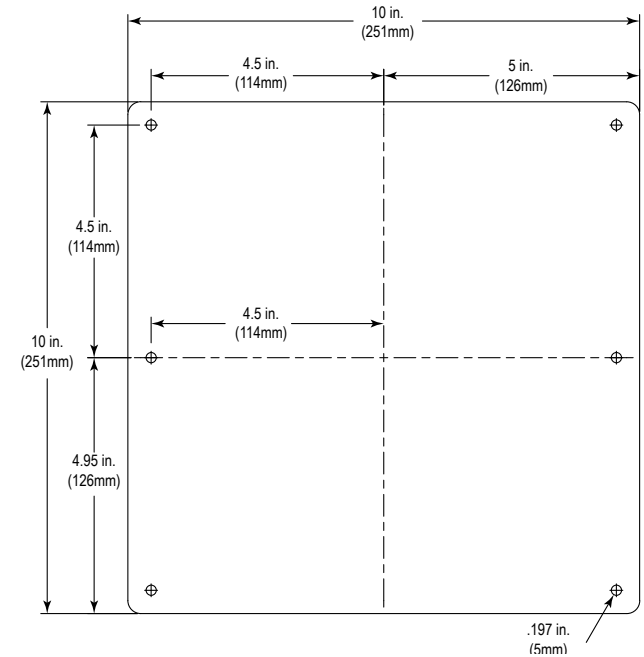
BACKPLATE STI-MBP1010
