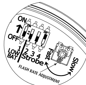
DETAIL S2
